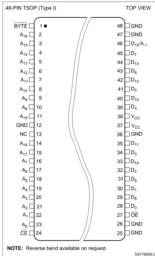
Figure 2. Pin Connections for TSOP (Type I) Package
