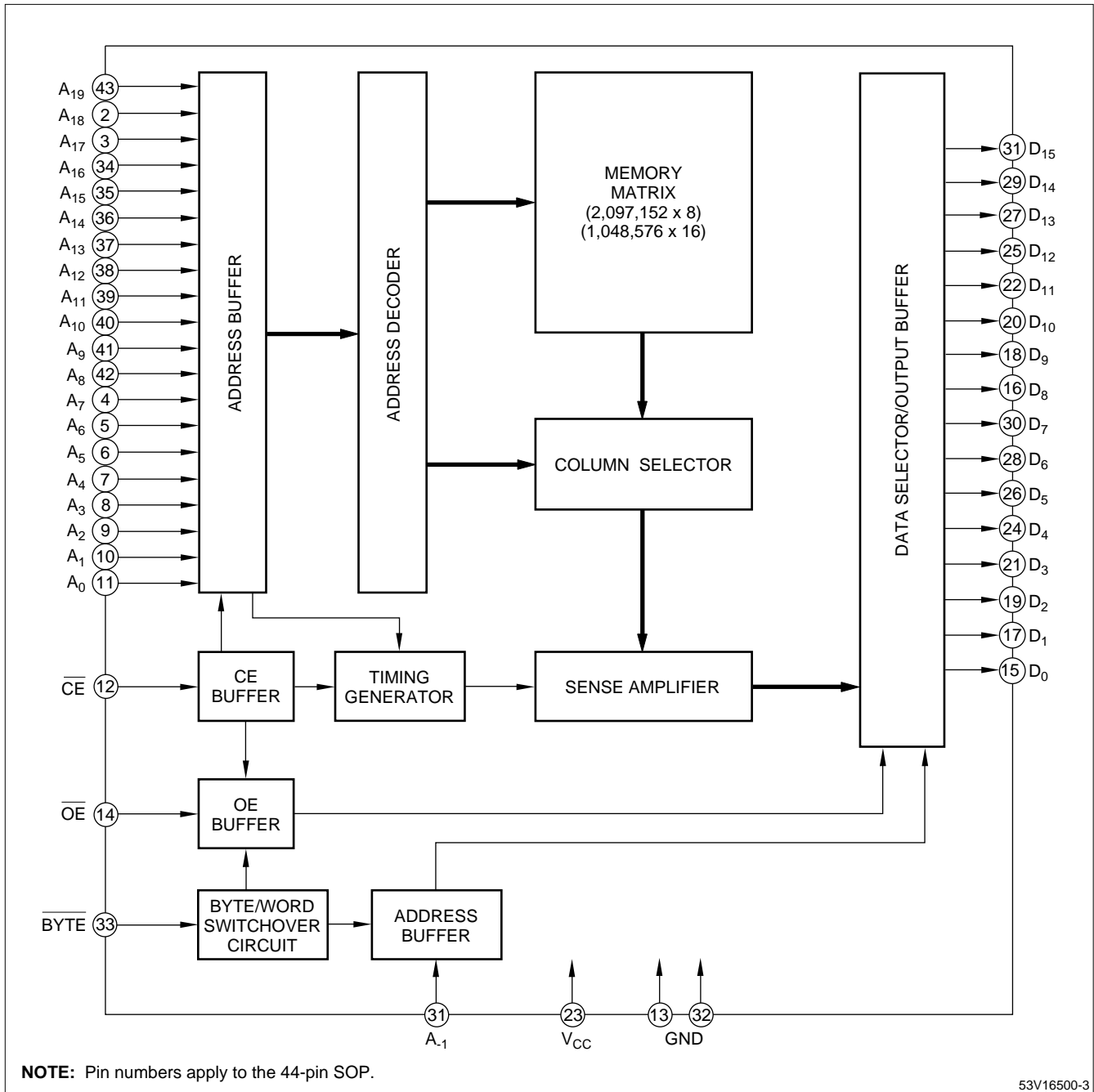
Figure 3. LH53V16500 Block Diagram
